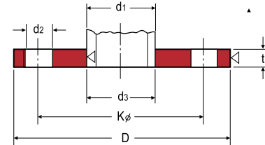
SLIP-ON/PLATE
