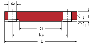
BLIND
