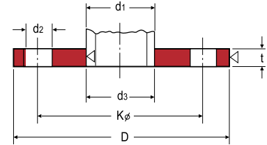
SLIP-ON/PLATE
