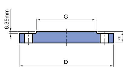
BLIND
