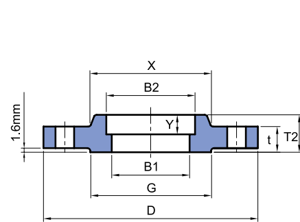
SOCKET WELDING
