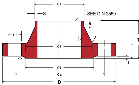
WELDING NECK
