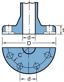
SOLID FLANGE
