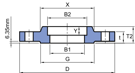
SOCKET WELDING
