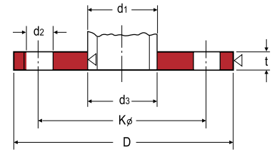
SLIP-ON/PLATE
