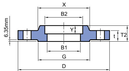
SOCKET WELDING
